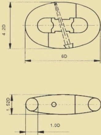
KENTER SHACKLE=KS
