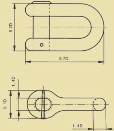
ANCHOR SHACKLE=A. S
