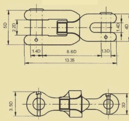
ANCHOR SWIVEL SHACKLE (b)=A.SW.S (b)
