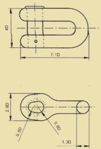
JOINING SHACKLE=JS
